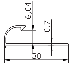
FC-5349 0.092 kg/m
